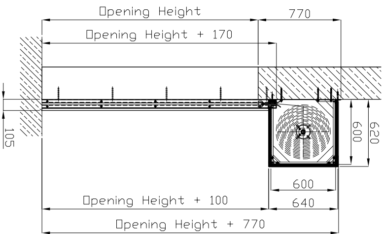
Type 4 housing.
