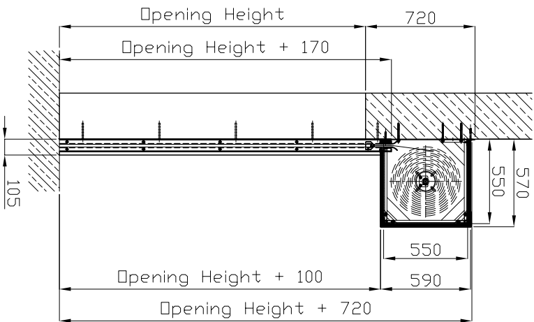
Type 3 housing.
