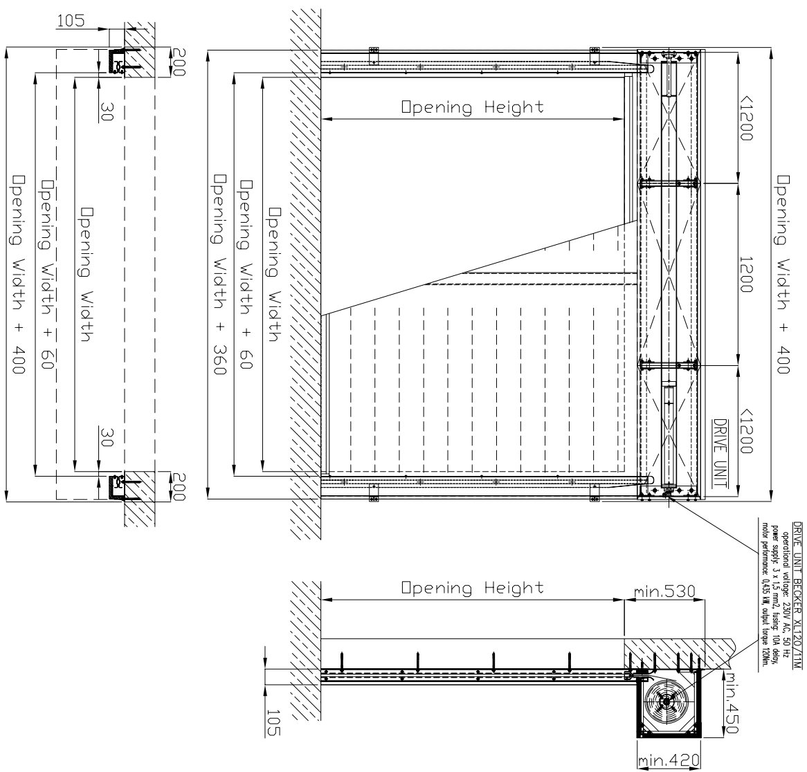
Type 2 housing.
