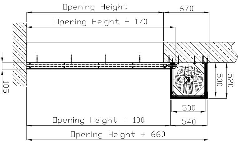
Type 2 housing.
