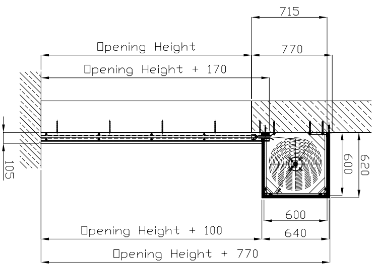
Type 4 housing.
