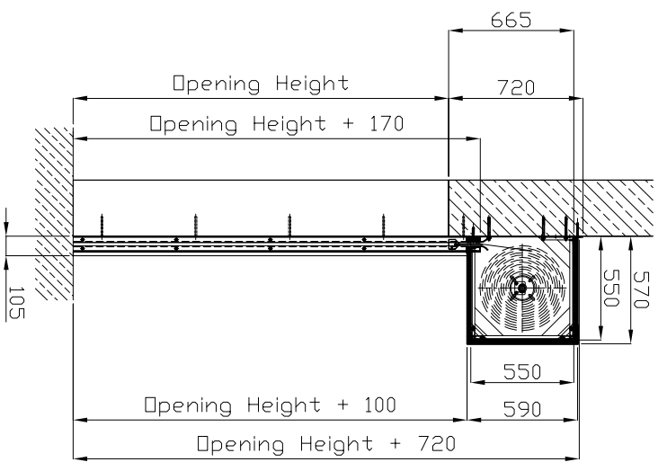
Type 3 housing.
