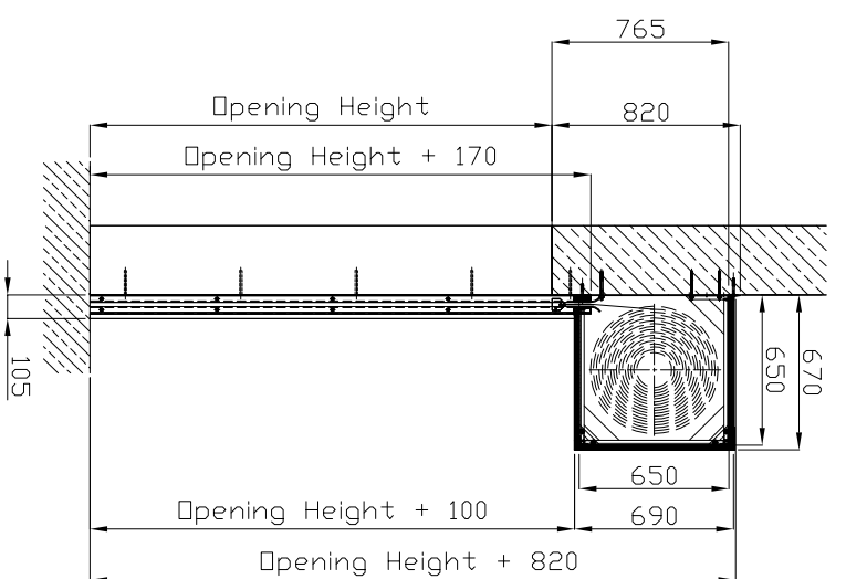
Type 5 housing.
