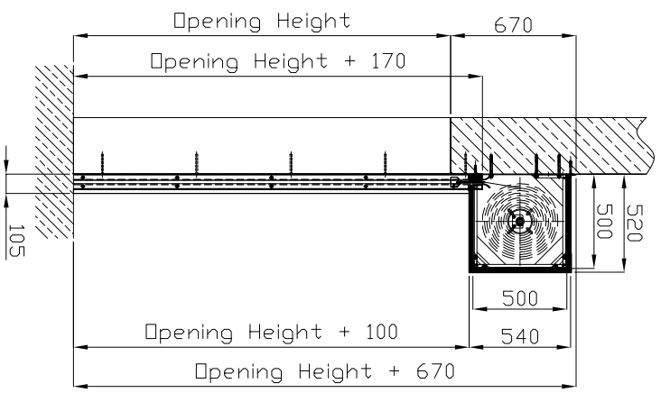
Type 2 housing.
